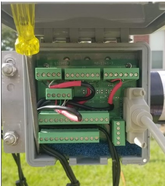
SteppIR Interface Box
